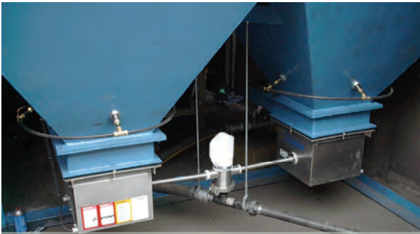
Volumetric Feeder & Eductor Transfer System Delivering Magic Powder To Treat Baghouse Containing Hazardous Dusts
